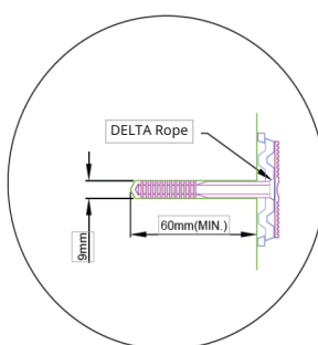
ULTRA FIX PLUG FIXING DETAILS
